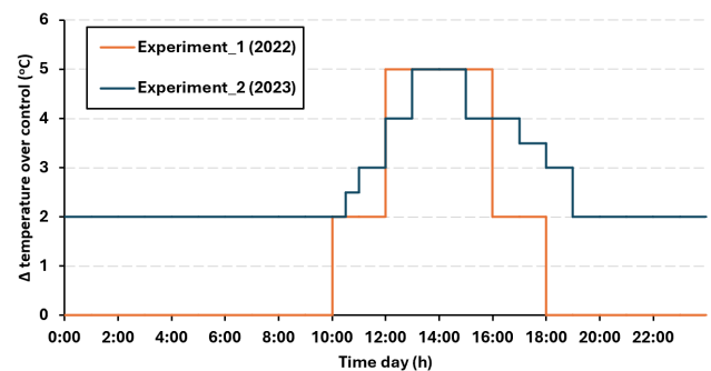
Figure 3. Warm-up regimen based on the time of day. Treated plots were heated by a theoretical air temperature differential (see Supplementary Material S3 for details) with reference to the control plots, depending on the time of day. Temperature regimes varied for each experiment according to the heat wave intended to be simulated.
