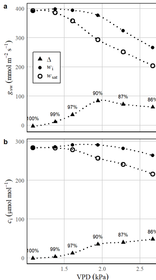
Figure 3. Computation of stomatal conductance ( g_{sw} ) and substomatal CO_2 concentration ( c_i ) assuming saturation in the substomatal cavity ( w_{sat} ) and accounting for actual vapour concentration ( w_i ) as a function of atmospheric vapour pressure deficit (VPD). (a) g_{sw} plotted against VPD, comparing the calculations for w_{sat} (open circles) and w_i (filled circles). The triangles represent the difference ( \Delta ) between these calculations. (b) c_i plotted against VPD, with the same model comparisons as in panel (a). The percentages at the top of the triangles indicate the relative humidity (RH) in the substomatal cavity calculated as the ratio of w_i/w_{sat} . The species used in this example is cotton. Data sourced from Wong et al. (2022).
