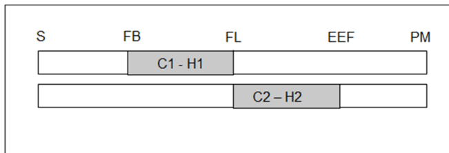
Figure 1. Schematic representation of the heating and control treatments conducted in Experiments 1 and 2 using control (C1-C2) and heating (H1-H2) portable structures during the pre-flowering (C1-H1) and post-flowering (C2-H2) phases. Gray bars indicate the periods when the corresponding treatments were applied. S = sowing, FB = flower-bud stage, FL = flowering stage, EEF = end of effective flowering stage or cut-out, PM = physiological maturity.
