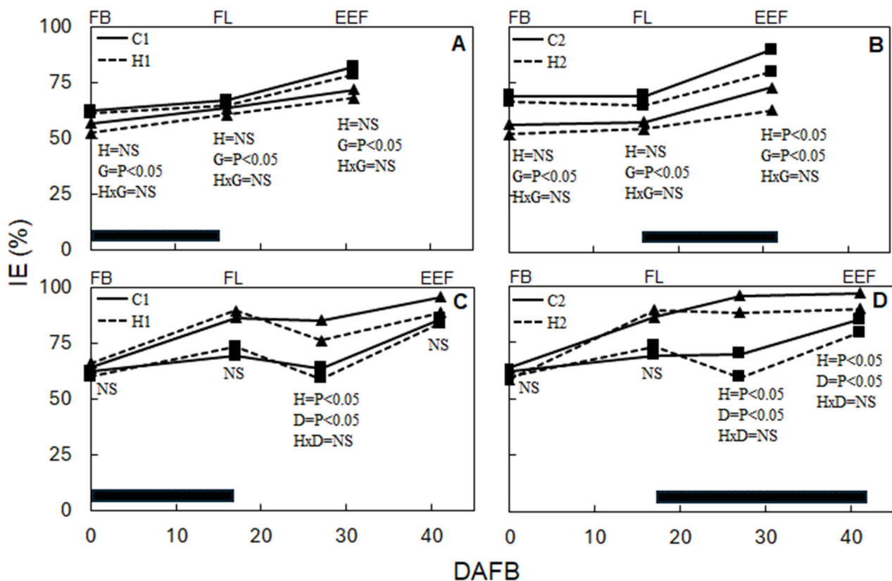
Figure 3. Interception efficiency (IE) as a function of the days after the onset of the flowering-bud stage (DAFB), for the short (Gs, ▲) and long (G1, ■) genotypes, in Experiment 1 (A,B) and for the non-defoliated (D0, ▲) and defoliated (D-, ■) treatments in Experiment 2 (C,D), subjected to control (entire lines) and heat (dotted lines) temperature treatments. Horizontal black bars indicate the period covered by the treatments between FB and flowering (FL) and between FL and the end of the effective flowering period or cut-out (EEF) for pre-flowering (A,C) and post-flowering (B,D) treatments, respectively. Two-way ANOVA analyses were performed for each measuring date and the results are indicate inside the Figure. H = temperature treatments, G = genotype, D = defoliation treatments, NS = non-significant.
