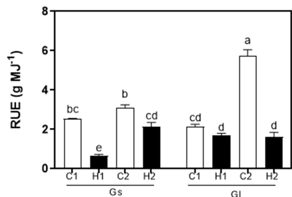
Figure 4. Radiation use efficiency (RUE, g MJ^{-1} ) estimated for the period FB-FL (pre-flowering; C1-H1) and FL-EEF (post-flowering; C2-H2) for control (C1-C2) and heat (H1, H2) treatments. Data are presented for the short cycle (Gs) genotype DP402 and the long cycle (Gl) genotype DP1238 in Experiment 1. Vertical bars are standard errors for means ( n = 9 ) and different letters indicate significant differences among treatments ( p < 0.05 ).
