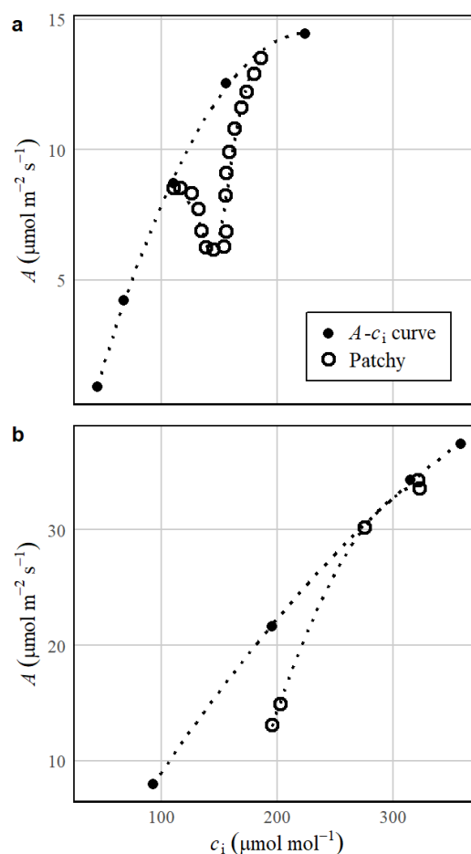
Figure 4. The effect of stomatal patchiness on the assimilation rate ( A ) vs. \text{CO}_2 concentration in the substomatal cavity ( c_i ) relationship ( A - c_i ). (a) Filled circles represent the A - c_i curve under steady-state and benign conditions. Open circles show how patchy stomatal closure distorts this curve over time after ABA application to induce patchiness in Malus dolgo . Time progression in the open circles moves from right to left. Data from Mott (1995). (b) Filled circles represent the A - c_i curve under steady-state and benign conditions, while open circles show steady-state measurements at elevated VPDs to induce patchiness in Helianthus annuus . Data sourced from Márquez et al. (2023a). The VPD increase imposed for each open circle in panel (b) was 1, 1.2, 1.5, 2, and 2.5 kPa, progressing from right to left as depicted in the figure.
