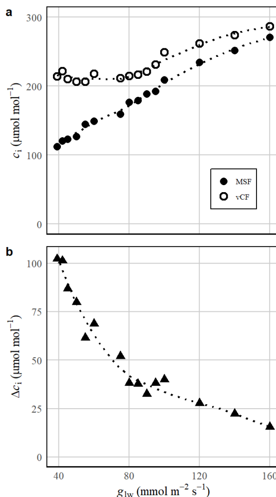
Figure 2. Estimation of substomatal \text{CO}_2 concentration ( c_i ) as a function of total leaf surface conductance to water ( g_{lw} = \text{stomatal conductance} + \text{cuticular conductance} ). (a) Substomatal \text{CO}_2 concentration ( c_i ) plotted against changes in g_{lw} , which follow the leaf's circadian rhythm. The comparison includes two models to estimate c_i : one that accounts for small fluxes (MFS, solid circles) and one that does not (vCF, open circles). (b) The difference in c_i ( \Delta c_i = \text{vCF} - \text{MFS} , solid triangles) between the two models is plotted against g_{lw} . Measurements were conducted under constant light, vapour pressure deficit, and ambient \text{CO}_2 concentration. The estimated cuticular conductance for this leaf is 10 \text{ mmol m}^{-2} \text{ s}^{-1} . Data sourced from Márquez, Stuart-Williams and Farquhar (2021). Each point represents a single measurement, calculated independently using the vCF and MFS models.
