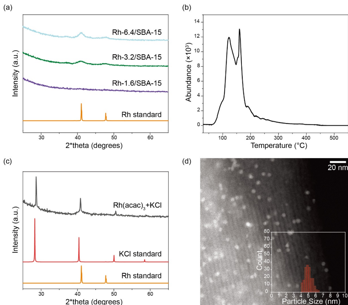
Figure 2. Characterization of the Rh-X/SBA-15 catalysts and the effect of \text{Cl}^- from KCl on the size of Rh NPs. (a) PXRD patterns for each NP size. (b) \text{H}_2 -TPR of un-reduced \text{RhCl}_3/\text{SBA-15} . (c) PXRD and (d) STEM of \text{Rh}(\text{acac})_3/\text{SBA-15} reduced in the presence of KCl with a ratio of \text{Rh}:\text{Cl} = 1:3 . Inset in (d) is the size histogram of Rh NPs. Reduction condition: 10% \text{H}_2 in He was flowed at 50 mL/min, starting at 30 °C and ramping at 5 °C/min.
