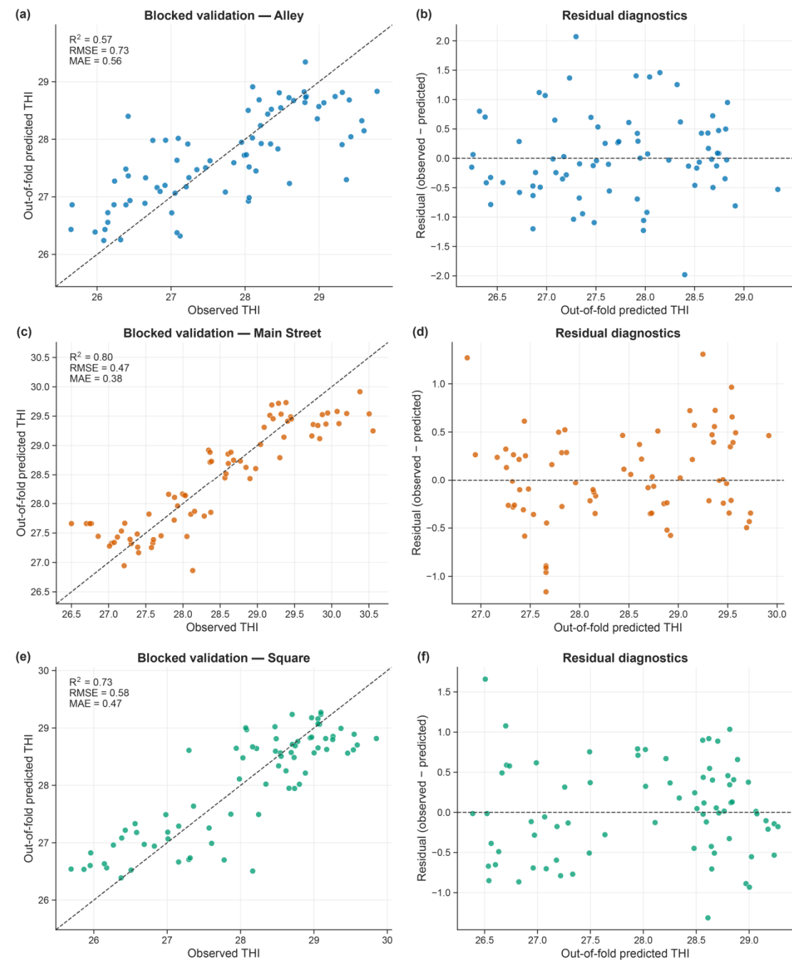
Figure S1. Grouped block cross-validation performance and residual diagnostics of XGBoost models across three analytical scenarios. Observed versus out-of-fold predicted THI and corresponding residual diagnostics for (a,b) the reconstructed Alley scenario, (c,d) Main Street, and (e,f) Square. Dashed lines in panels (a), (c), and (e) represent the 1:1 relationship; dashed horizontal lines in panels (b), (d), and (f) indicate zero residual. R^2 , RMSE, and MAE were calculated from grouped out-of-fold predictions.
