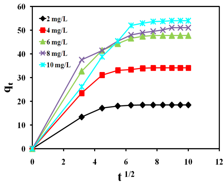
Figure S1. Weber-Morris plots for fluoride adsorption by NAAC.
