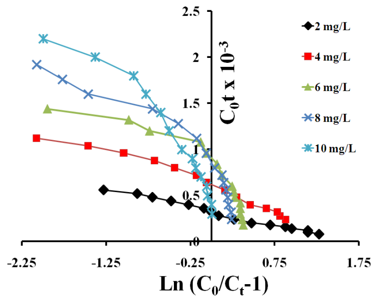
Figure S2. BDST plots for the removal of fluoride concentrations by NAAC.
