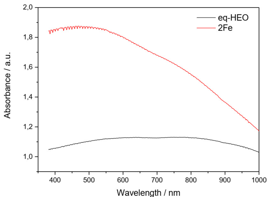
Figure S3. UV-Vis absorbance spectra measured on two aqueous solutions with the same load ( 0.235 \text{ g L}^{-1} ) of 2Fe and eq-HEO PCs.
