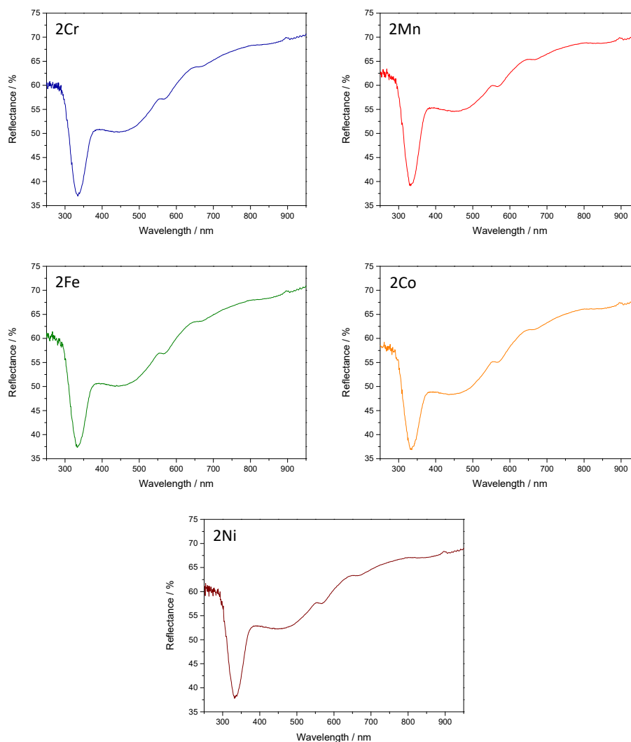
Figure S1. Reflectance spectra of investigated HEOs.
