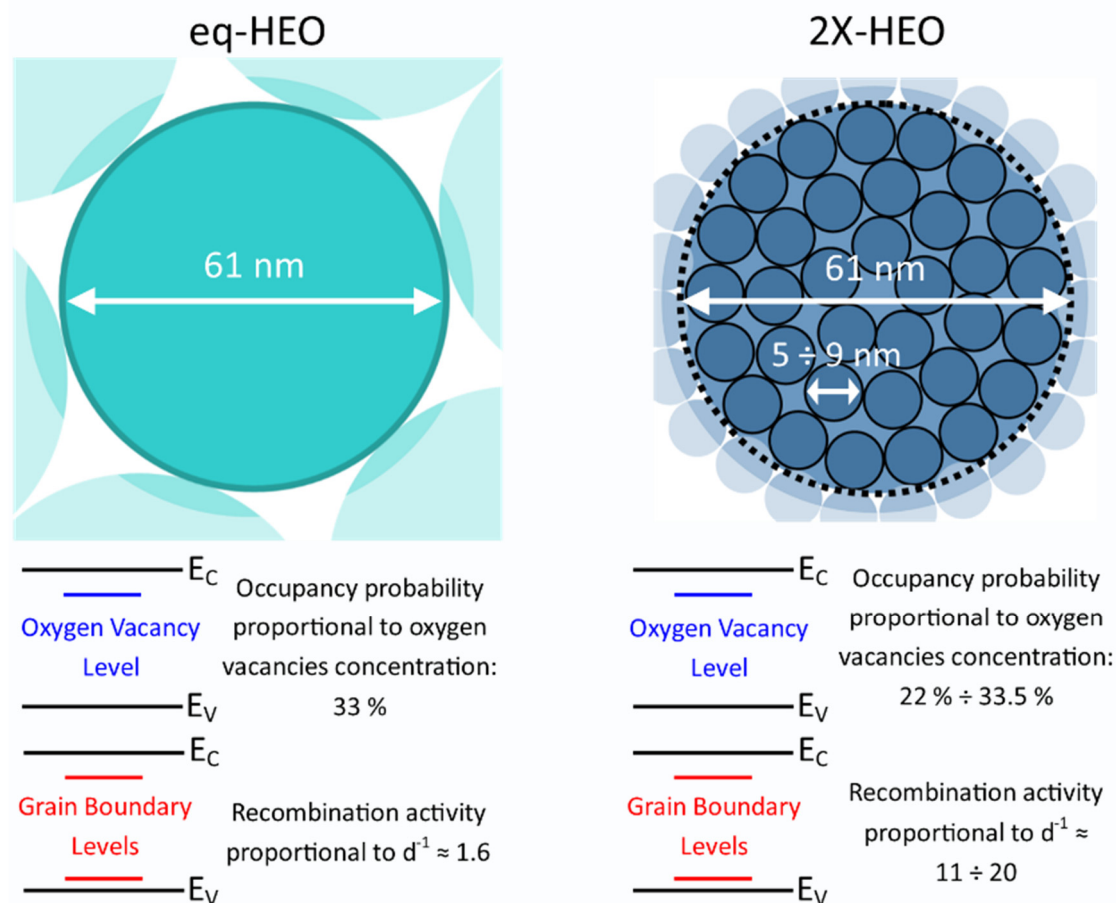
Figure S2. GB density as a function of size of HEO nanoparticles.
