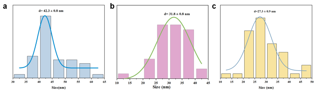
Figure S1. The particle size distribution graphs of \text{Cu}_1\text{Mg}_0 (a), \text{Cu}_1\text{Mg}_1 (b), and \text{Cu}_0\text{Mg}_1 (c).
