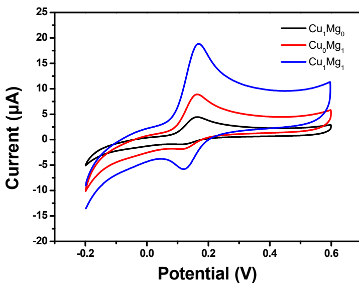
Figure S2. CV curves of \text{Cu}_x\text{Mg}_y catalysts in [\text{Fe}(\text{CN})_6]^{3-/4-} solution.
