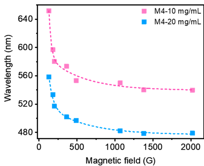
Figure S3. The reflection peak wavelength and structural color comparison of sample M4 with concentrations of 10 mg/mL and 20 mg/mL upon exposure to magnetic fields.
