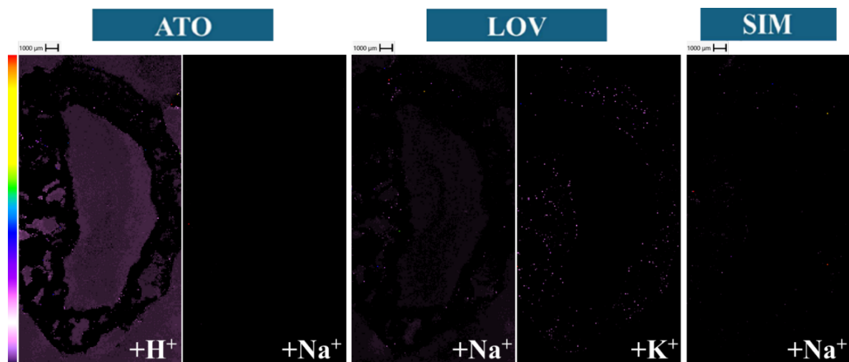
Figure S1: Distribution of Statins in Control Earthworms. Earthworms were exposed to equal volumes of water as opposed to statin dosing solution. The images shown here represent the signal generated by an adduct of the statin parent compound normalized to the TIC. The appropriate adduct is indicated in the lower right corner of each image.
