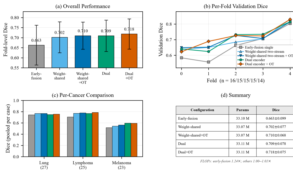
Figure 2. Summary of the 200-epoch comparison across five of the six configurations of Table 1, omitting the dual encoder with the original non-differentiable OT term. (a) Fold-level mean Dice, with the SD taken over the five folds. (b) Per-fold validation Dice; the ranking of the configurations reverses between folds. (c) Per-cancer Dice, pooled per case. (d) Parameter counts and fold-level mean Dice. Every value is computed from the same artifacts as Tables 1 and 2. The two matched-capacity control configurations are specified in Section 3.2; neither is the original 22 M baseline encoder, and their parameter counts are given in panel (d).
