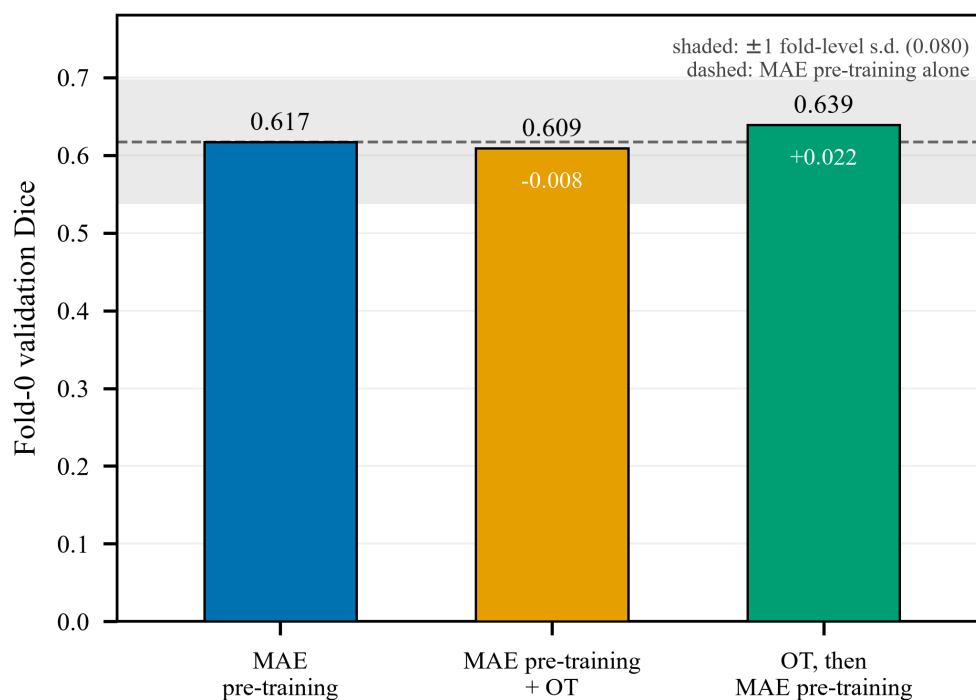
Figure 5. Single-fold (fold 0) MAE and OT interaction at 200 epochs. The MAE and OT combination is 0.008 below MAE alone and the reverse ordering is 0.022 above it, so the data do not establish an antagonistic interaction.
