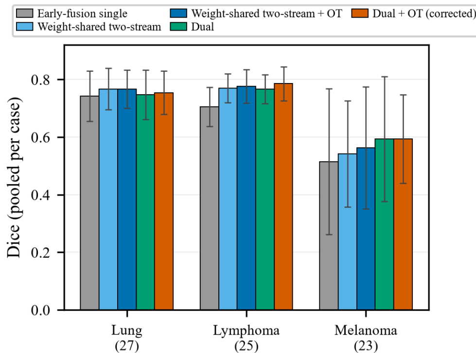
Figure 4. Per-cancer Dice across the five 200-epoch configurations of Table 2. Melanoma is both the lowest-scoring and the most dispersed of the three cancer types. Error bars are the SD over the five fold means, the same dispersion the table reports beside each cancer type.
