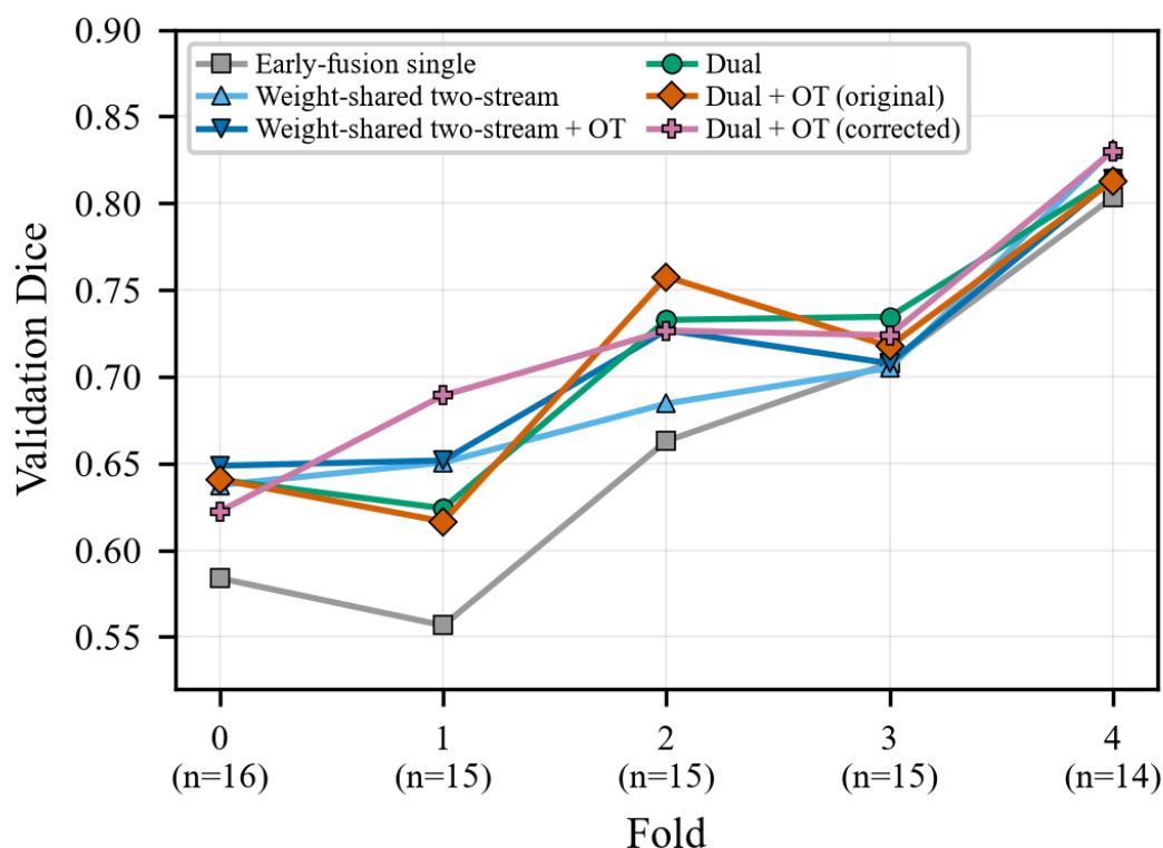
Figure 8. Per-fold validation Dice across the five splits, for the six configurations of Table 1. The rankings reverse between folds, so no configuration dominates across partitions. Fold sizes are 16, 15, 15, 15 and 14 cases, and the folds are not stratified by cancer type.
