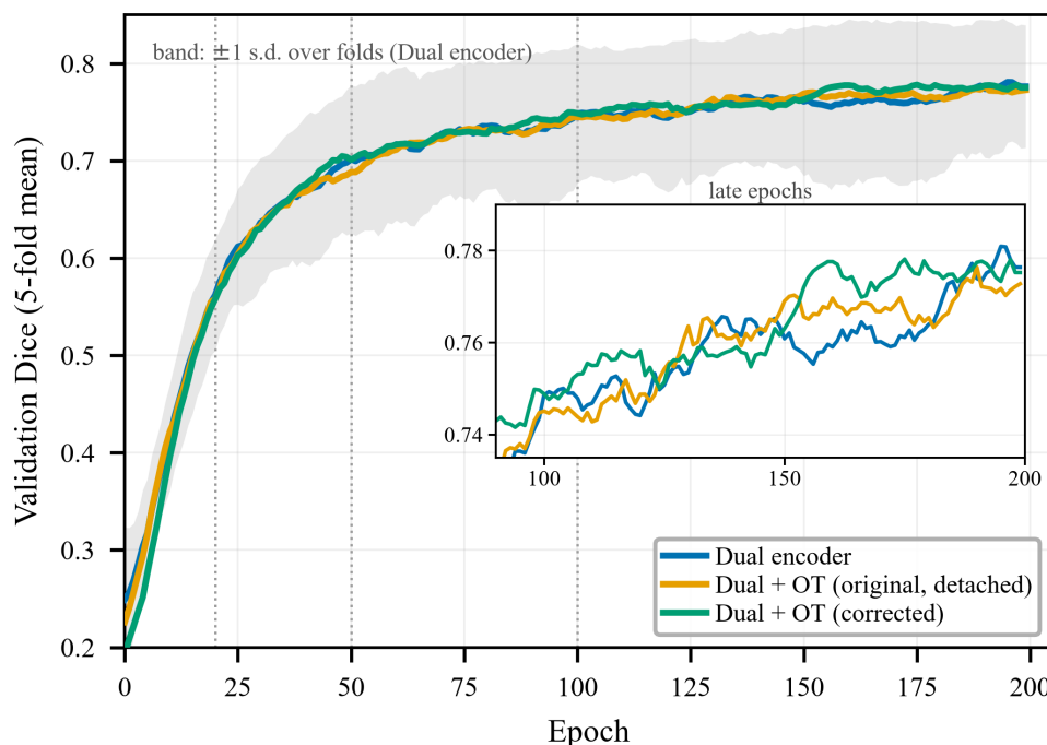
Figure 3. Five-fold mean validation Dice over the full 200-epoch schedule for the three dual-encoder configurations; the vertical axis is the patch-level Dice computed on the validation patches during training, not the per-case Dice reported in Table SI—for the dual encoder without OT the two read 0.776 and 0.709 on the same runs. The shaded band is one SD over the folds for the dual encoder without OT. Against the original, non-differentiable OT term the largest separation is 0.0132 Dice at epoch 50, with the OT arm behind. The corrected, differentiable OT term is not separated either: after the tenth epoch it stays within 0.021 Dice of the no-OT arm at every epoch. Neither separation is significant (inset, late epochs).
