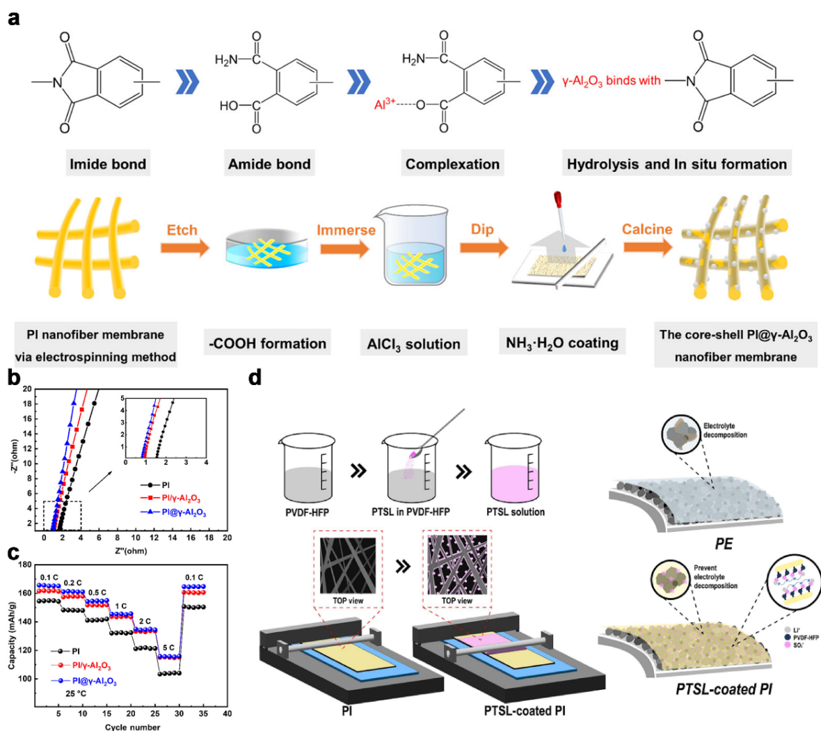
Figure 10. (a) Schematic illustrating the synthesis of the core-shell \text{PI}@\gamma\text{-Al}_2\text{O}_3 nanofiber membrane. Electrochemical performance of cells with different separators: (b) impedance profiles and (c) discharge capacities at various C-rates. Reproduced with permission [80]. Copyright 2023, American Chemical Society. (d) Coating process for preparing PTSL-modified PI. Reproduced with permission [83]. Copyright 2024, The Korean Society of Industrial and Engineering Chemistry. Published by Elsevier B.V.
