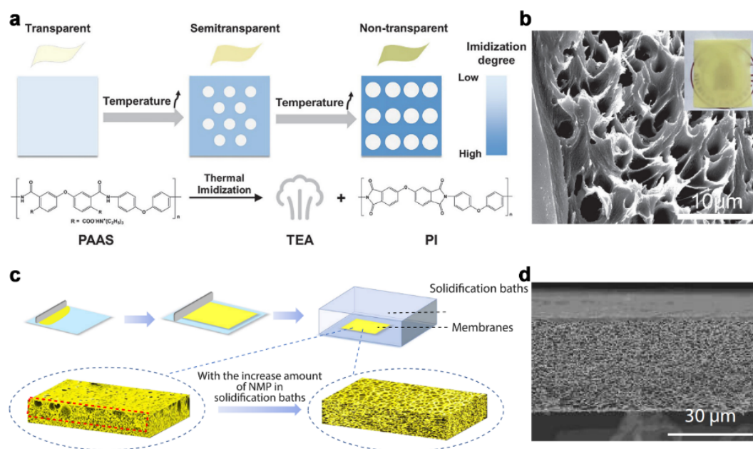
Figure 1. (a) Illustration depicting the morphological transition from a PAAS film to a PI film. (b) Cross-sectional SEM micrographs of the films processed at 220^\circ\text{C} , accompanied by their corresponding optical images (inset). Reproduced with permission [43]. Copyright 2024, Elsevier B.V. (c) Process flow diagram illustrating the fabrication steps of PI separators. (d) Cross-sectional view of the PI-85:15 separator. Reproduced with permission [45]. Copyright 2022, Chinese Chemical Society Institute of Chemistry.
