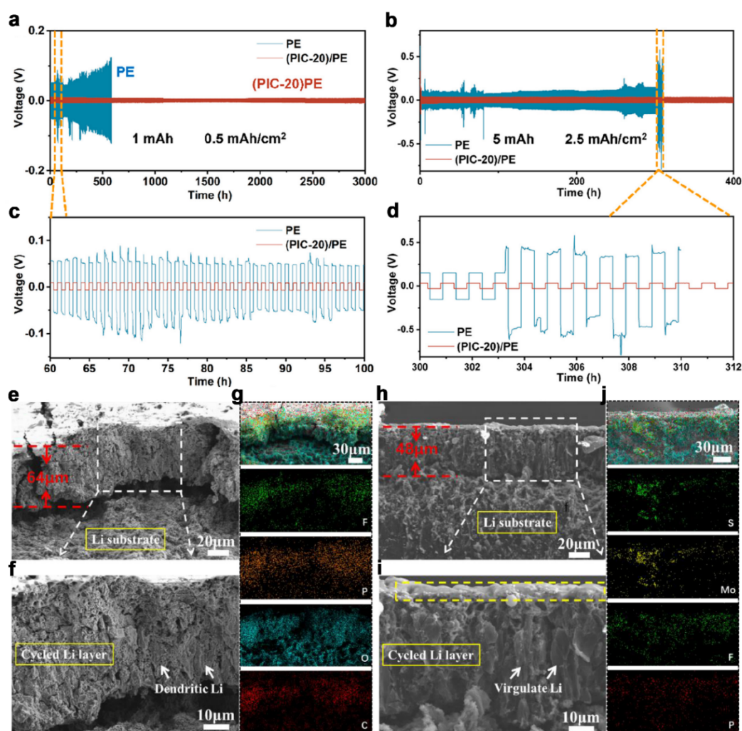
Figure 13. Electrochemical performance of symmetric Li/Li cells employing (PIC-20)/PE separators. Voltage-time profiles for cells with area capacities of (a,c) 0.5\text{ mAh cm}^{-2} and (b,d) 2.5\text{ mAh cm}^{-2} , comparing PE and (PIC-20)/PE separators. Reproduced with permission [25]. Copyright 2023, American Chemical Society. SEM characterization of Li anodes after 100 cycles ( 1\text{ mA cm}^{-2} , 1\text{ mAh cm}^{-2} ). (e,f) Cross-sectional views at low and high magnification, and (g) corresponding EDS analysis of the pure Li electrode. (h,i) Cross-sectional views at low and high magnification, and (j) associated EDS analysis of the Li electrode paired with the composite separator. Reproduced with permission [93]. Copyright 2022, Elsevier Ltd. on behalf of The editorial office of Journal of Materials Science & Technology.
