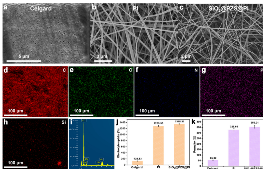
Figure 4. (a–c) The morphologies of Celgard, PI, and SiO 2 @PZS@PI separators are shown in the SEM images. (d–h) The elemental distribution and (i) EDS result are provided for the SiO 2 @PZS@PI sample. Furthermore, (j) the electrolyte uptake and (k) porosity of all separators are compared. Reproduced with permission [60]. Copyright 2025, American Chemical Society.
