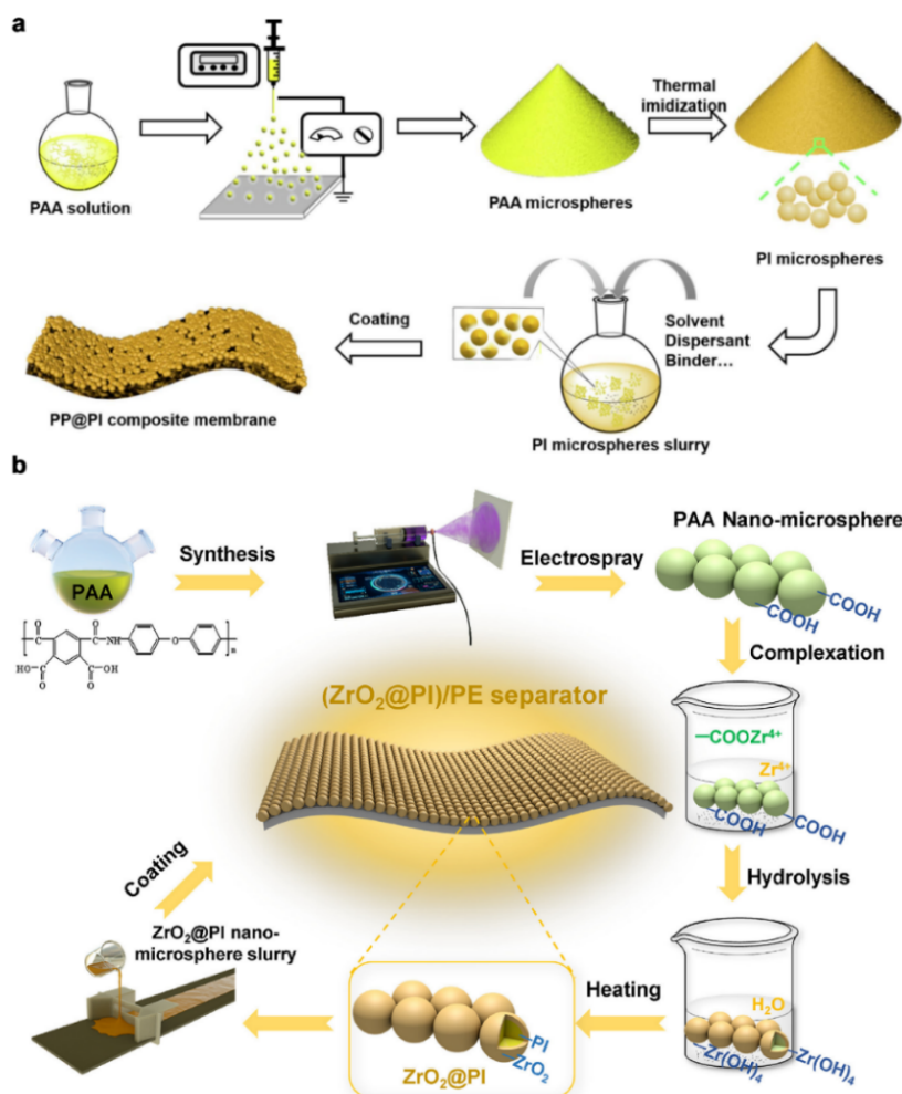
Figure 5. (a) Structural schematic of the PP@PI microsphere composite membrane. Reproduced with permission [18]. Copyright 2022, Elsevier B.V. (b) Preparation process of the ZrO 2 @PI core-shell nano-microsphere and the corresponding (ZrO 2 @PI)/PE separator via blade coating. Reproduced with permission [65]. Copyright 2022, Elsevier Ltd.
