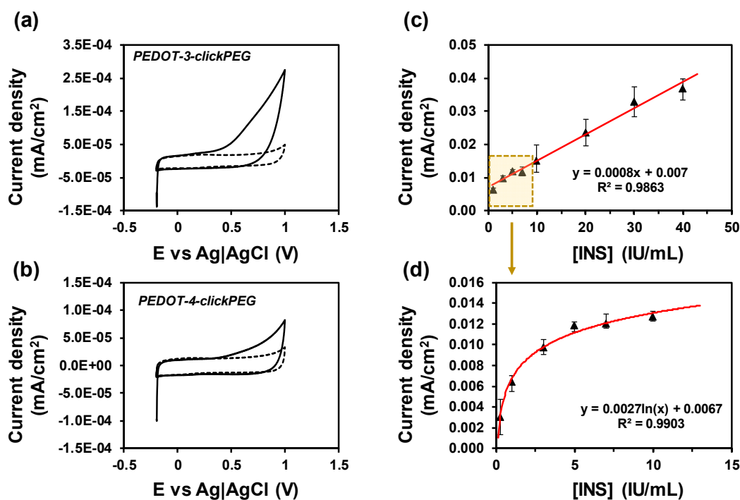
Figure 4. Electrochemical characterization of PEDOT-#-clickPEG hydrogels. Representative 3rd CV curve for (a) PEDOT-3-clickPEG and (b) PEDOT-4-clickPEG hydrogels. Dashed line corresponds to the blank hydrogel system (no PEDOT; 3-clickPEG or 4-clickPEG, respectively). Calibration plot of oxidation peak current vs. INS concentration considering an interval up to (c) 40 IU/mL (the yellow rectangular indicates the data that is zoomed in (d) with an interval up to 10 IU/mL). Plots were obtained by CV using carbon SPE. Error bars represent standard deviations of three independent measurements.
